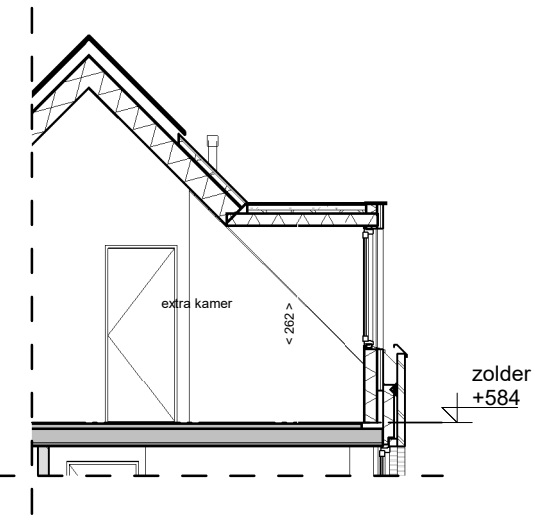
code 10600: dakkapel
